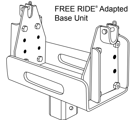
Detail of the "J" Bolt and Hardware installed into the FREE RIDE® Adapted Base Unit
